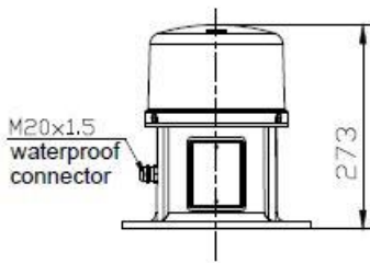
Connect drawing
