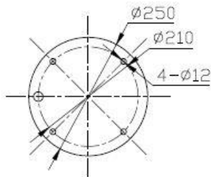
Installation (mm)
